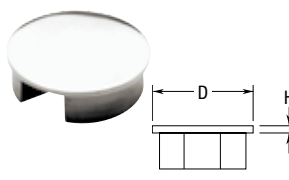
640 Channel Tube End Cap
