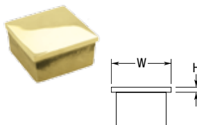
650 Flat Square End Cap
