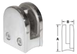
813R/2 1/2" GlassGrip™
