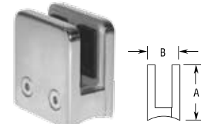
813/2 1/2" GlassGrip™
